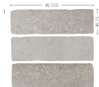
NF-B/RED-1 (Gray)
